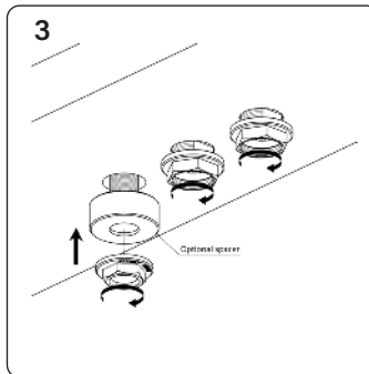
Fasten bodies
