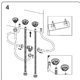
Install hoses
